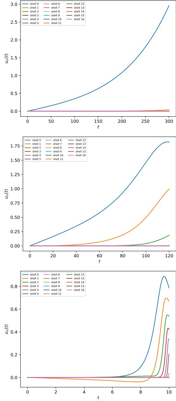
Fig. 8: Instanton solutions for z = \sum_n u_n = 3 at varying values of the nonlinear coupling: c_1 = 10^{-4} (top), c_1 = 10^{-2} (middle), and c_1 = 1 (bottom). All other parameters held fixed.
