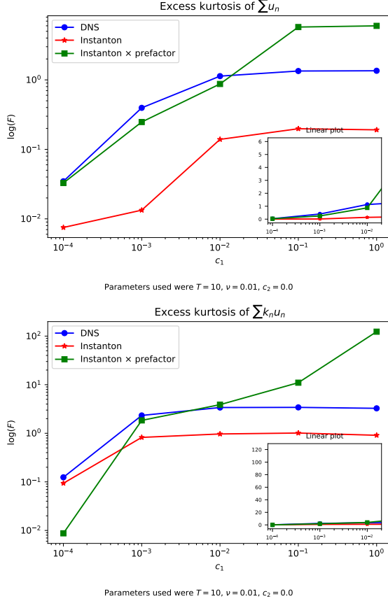
Fig. 10: Excess kurtosis plots for velocity (top) and velocity gradient (bottom) with respect to c_1 .
