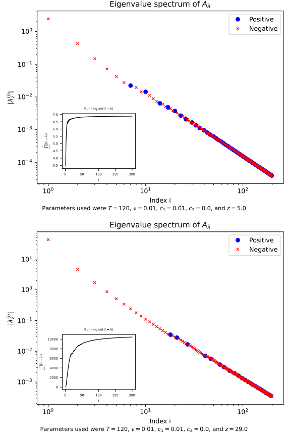
Fig. 9: Eigenvalue spectra with velocity as the target observable metric
