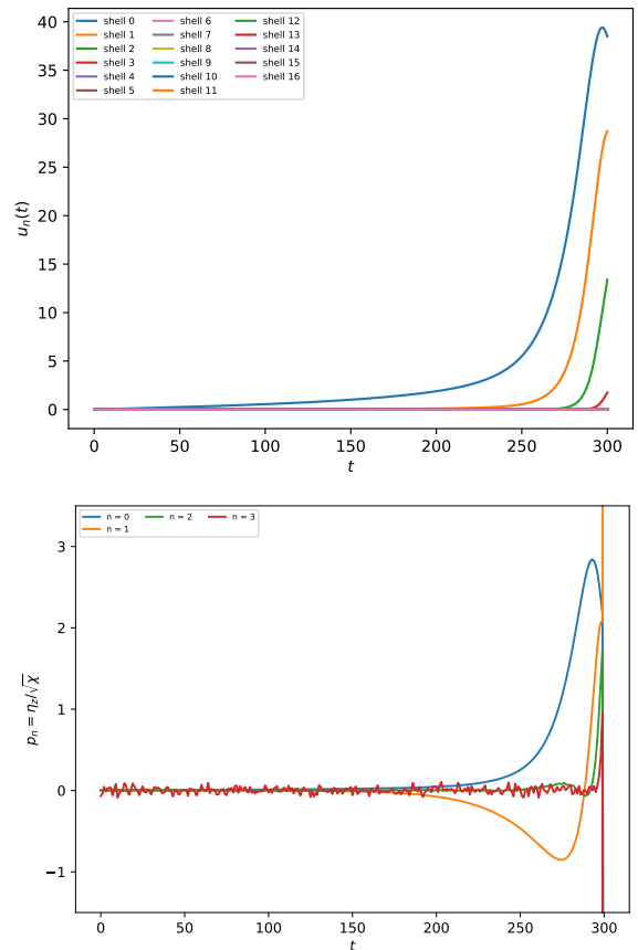
Fig. 6: The plots show the instanton solution for (12), adopting the same definition of p_n as is used in [2] for the plot on the bottom. The parameters used for these plots are z = \sum_n \langle u_n \rangle = 82.34 (corresponding to \lambda = 2 as in [2] Figure 5), c_1 = 10^{-3} , c_2 = 0.0 , \nu = 10^{-2} , and \chi_{nm} = k_n^{-6} \delta_{nm} .
